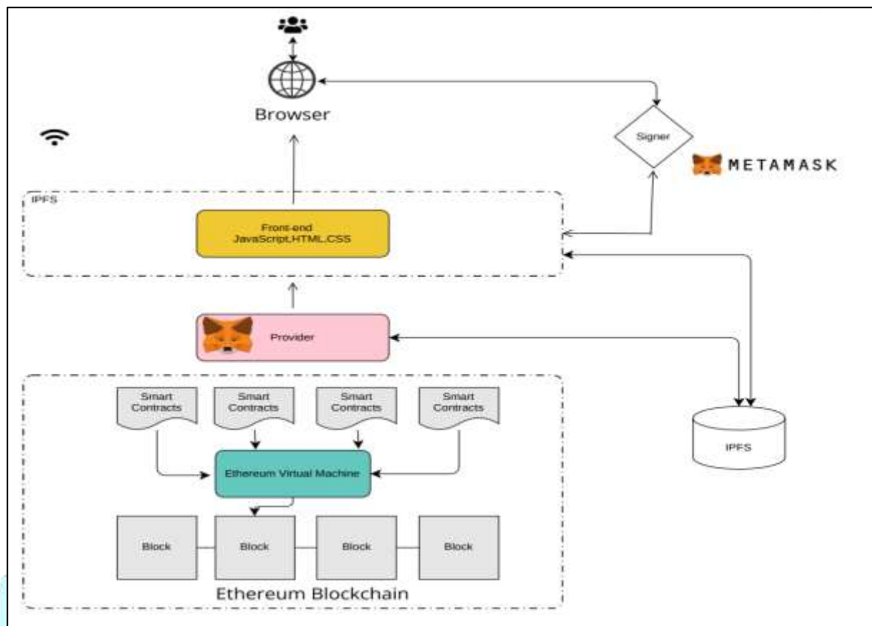
Figure 3: Internal structure of proposed application
