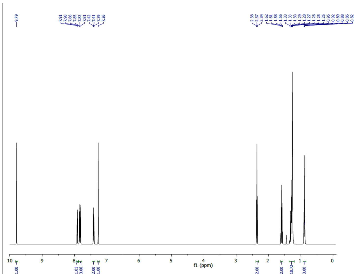
Figure S11: 1 H-NMR spectrum of C6 compound
