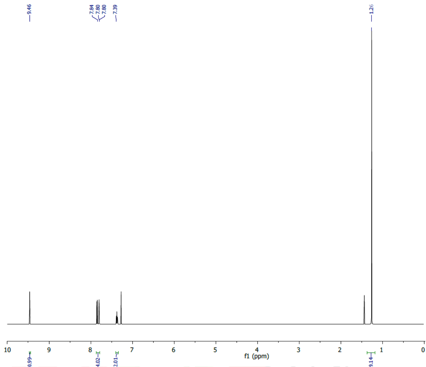
Figure S7: ^1\text{H} -NMR spectrum of C4 compound
