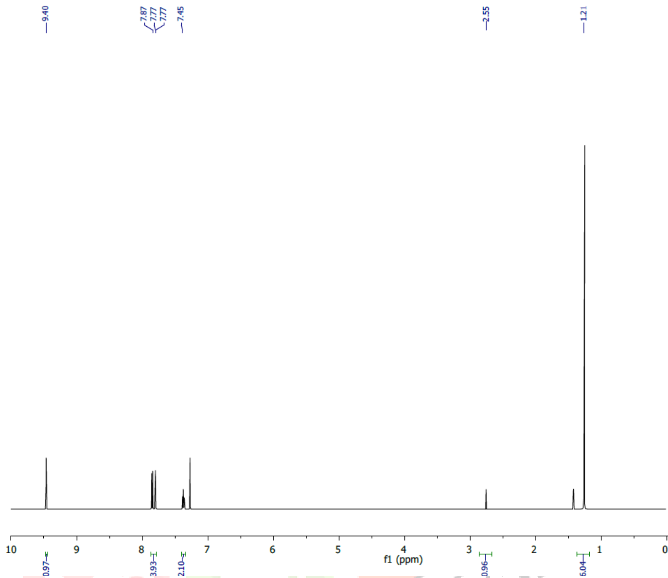
Figure S5: 1 H-NMR spectrum of C3 compound
