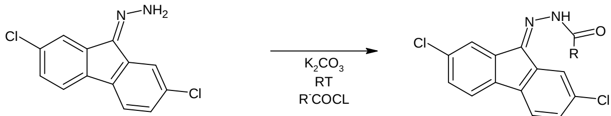
fig-2: synthesis of hydrazide from derived hydrazone
