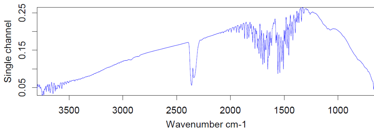
Figure S8: FTIR spectrum of C4 compound
