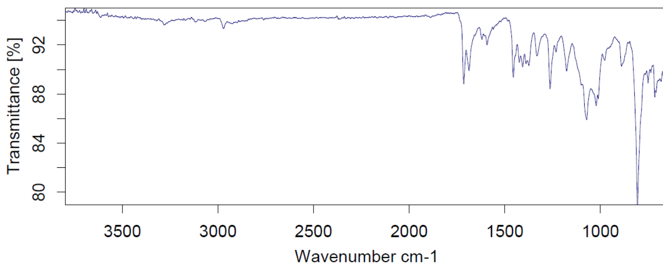
Figure S2: FTIR spectrum of C1 compound.
