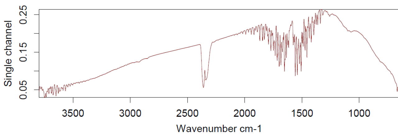
Figure S6: FTIR spectrum of C3 compound.
