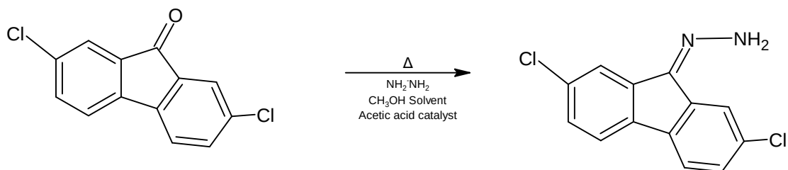
fig-1: synthesis of hydrazone from dichloro fluorenone
