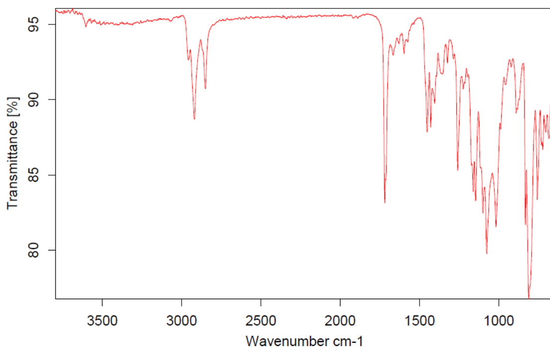
Figure S12: FTIR spectrum of C6 compound
