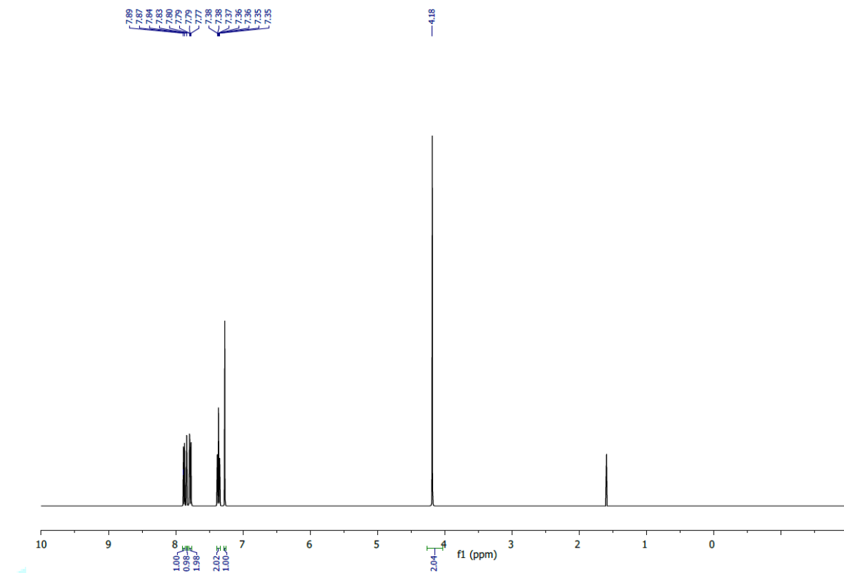
Figure S3: ^1\text{H-NMR} spectrum of C2 compound.
