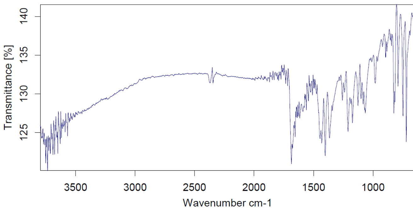
Figure S4: FTIR spectrum of C2 compound
