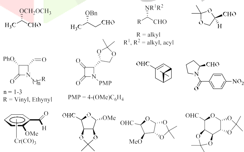
Fig. 2. Chiral electrophiles
