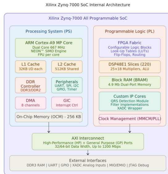
fig. 2. xilinx zynq-7000 soc internal architecture.
