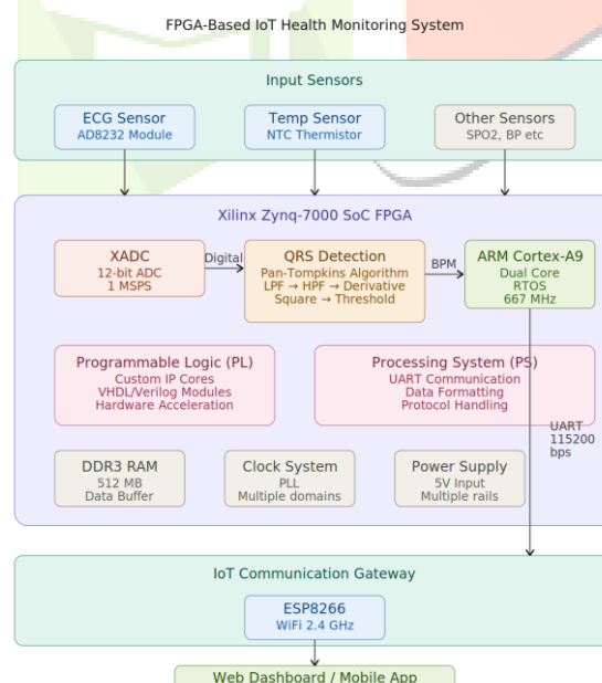
fig. 1. overall system block diagram.
