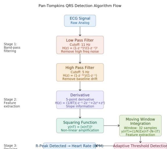
fig. 3. pan-tompkins qrs detection pipeline.
